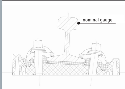
System DFF 21
