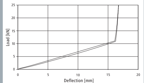
Load/spring deflection of tension clamp Skl 25
